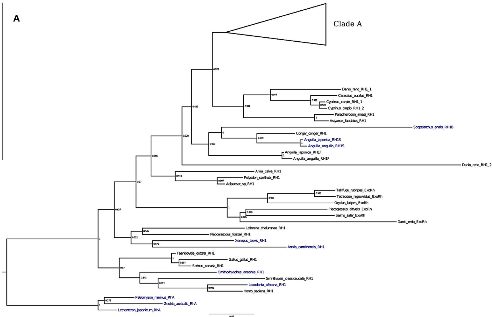
Fig. 4. Phylogenetic tree of RH1 opsins in fish. The tree was created using the maximum-likelihood method. Accession numbers are listed in Supplementary Table 1. RhA opsins from lamprey ( G. australis , P. marinus and L. japonicum ) were used as a root. PhyML was used to estimate genetic distances, based on Modeltest's best-fit model of evolution, and complete phylogenetic analysis (Guindon and Gascuel, 2003; Posada and Crandall, 1998). Tree topology was tested using the best of NNI and SPR. Numbers at nodes represent aLRT values (Anisimova and Gascuel, 2006). The model of evolution was determined to be GTR + I + G (I = 0.2746, G = 1.1396). Taxa names are color coded to show amino acid at position 83 (based on bovine rhodopsin numbering): black, aspartic acid; blue, asparagine. Clade A encompasses Euteleostei. (For interpretation of the references to color in this figure legend, the reader is referred to the web version of this article.)
