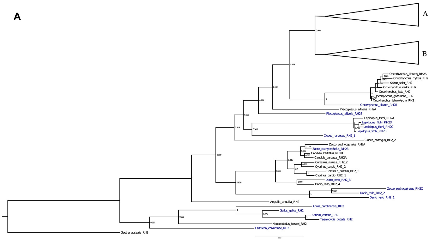
Fig. 5. Phylogenetic tree of RH2 opsins in fish. The tree was created using the maximum-likelihood method. Accession numbers are listed in Supplementary Table 1. RhB opsin from lamprey ( G. australis ) was used as a root. PhyML was used to estimate genetic distances, based on Modeltest's best-fit model of evolution, and complete phylogenetic analysis (Guindon and Gascuel, 2003; Posada and Crandall, 1998). Tree topology was tested using the best of NNI and SPR. Numbers at nodes represent aLRT values (Anisimova and Gascuel, 2006). The model of evolution was determined to be GTR + I + G ( I = 0.2485 , G = 0.8147 ). Taxa names are color coded to show amino acid at position 112 (based on bovine rhodopsin numbering): black, glutamic acid; blue, glutamine. The letters A and B indicate RH2A and RH2B clades respectively.
