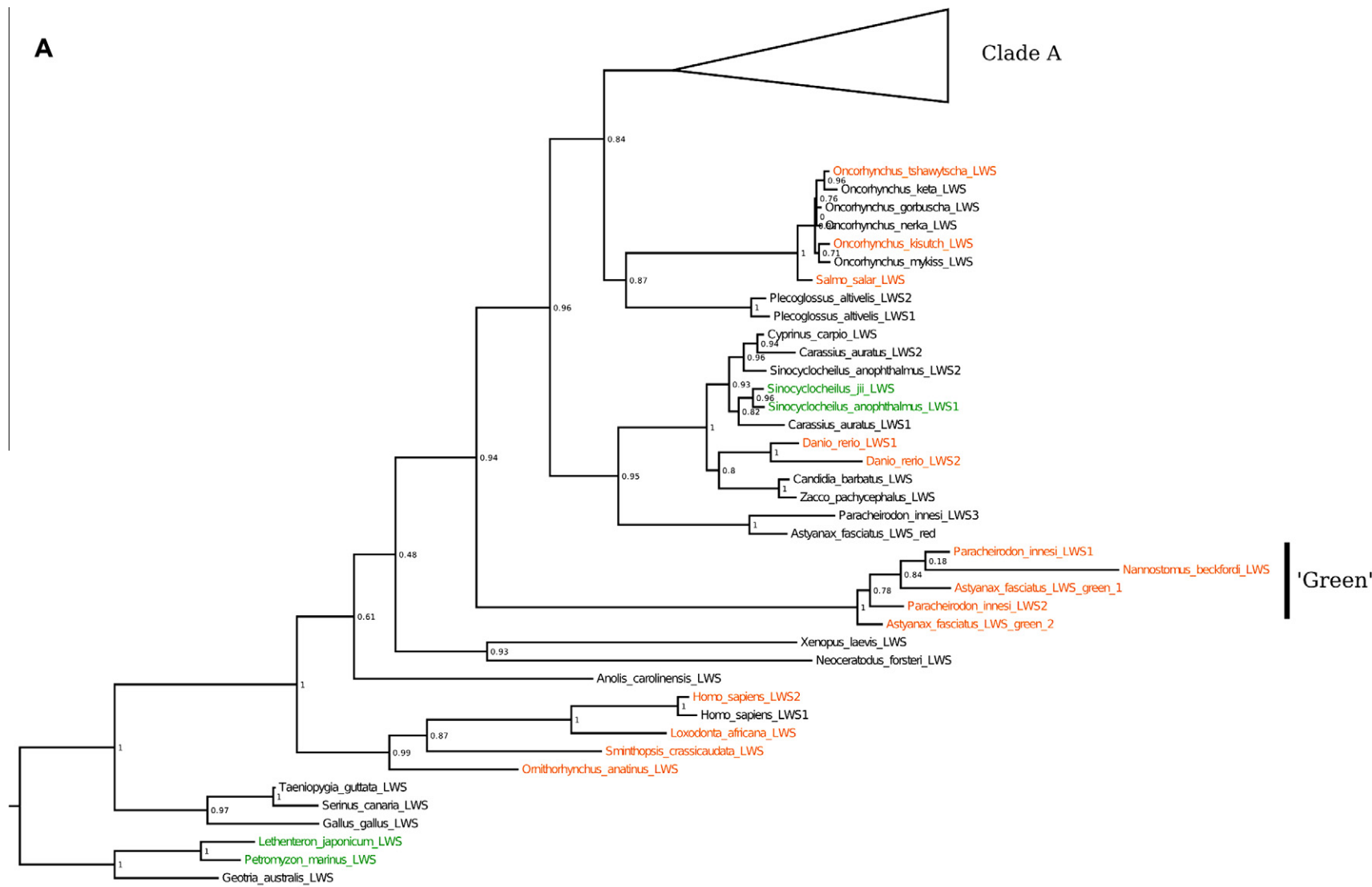
Fig. 6. Phylogenetic tree of LWS opsins in fish. The tree was created using the maximum-likelihood method. Accession numbers are listed in Supplementary Table 1. LWS opsins from lamprey ( G. australis , P. marinus and L. japonicum ) were used as a root. PhyML was used to estimate genetic distances, based on modeltest's best-fit model of evolution, and complete phylogenetic analysis (Guindon and Gascuel, 2003; Posada and Crandall, 1998). Tree topology was tested using the best of NNI and SPR. Numbers at nodes represent aLRT values (Anisimova and Gascuel, 2006). The model of evolution was determined to be GTR + I + G (I = 0.3378, G = 1.2425). The 'green' clade is indicated (see discussion). Taxa names are color coded to show amino acid at position 164 (based on bovine rhodopsin numbering): black, serine; orange, alanine; green, proline. Clade A encompasses Acanthopterygii.
